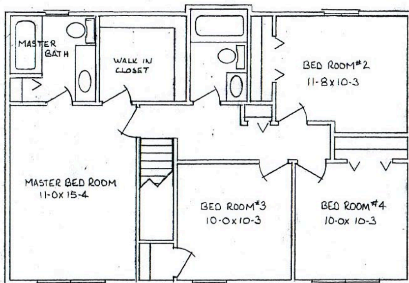
2nd Floor - 916 sq ft
